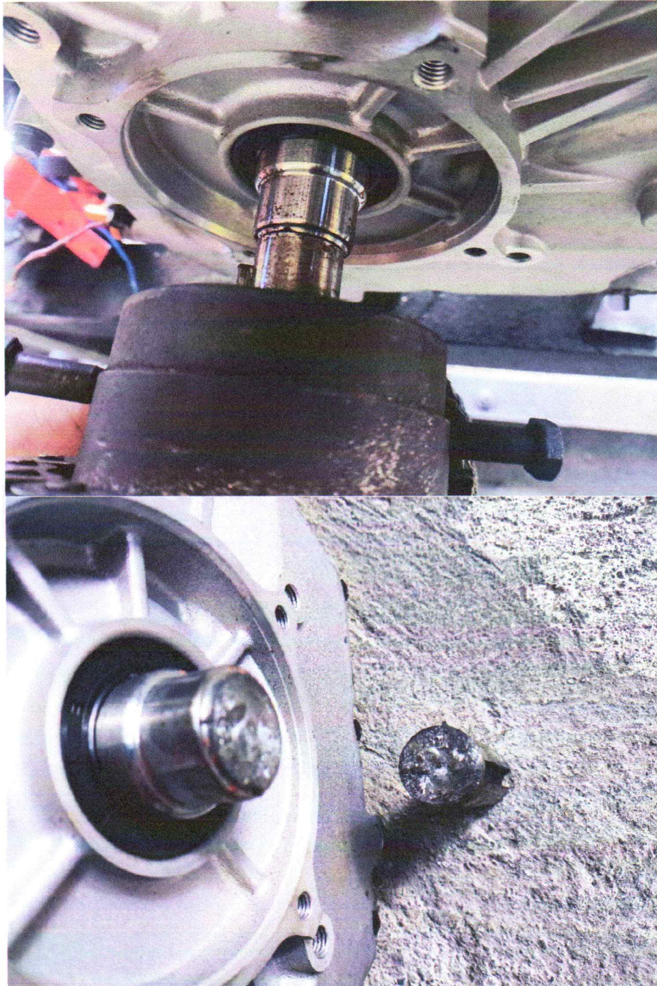
Figure 1. Observed engine shaft had snapped.
