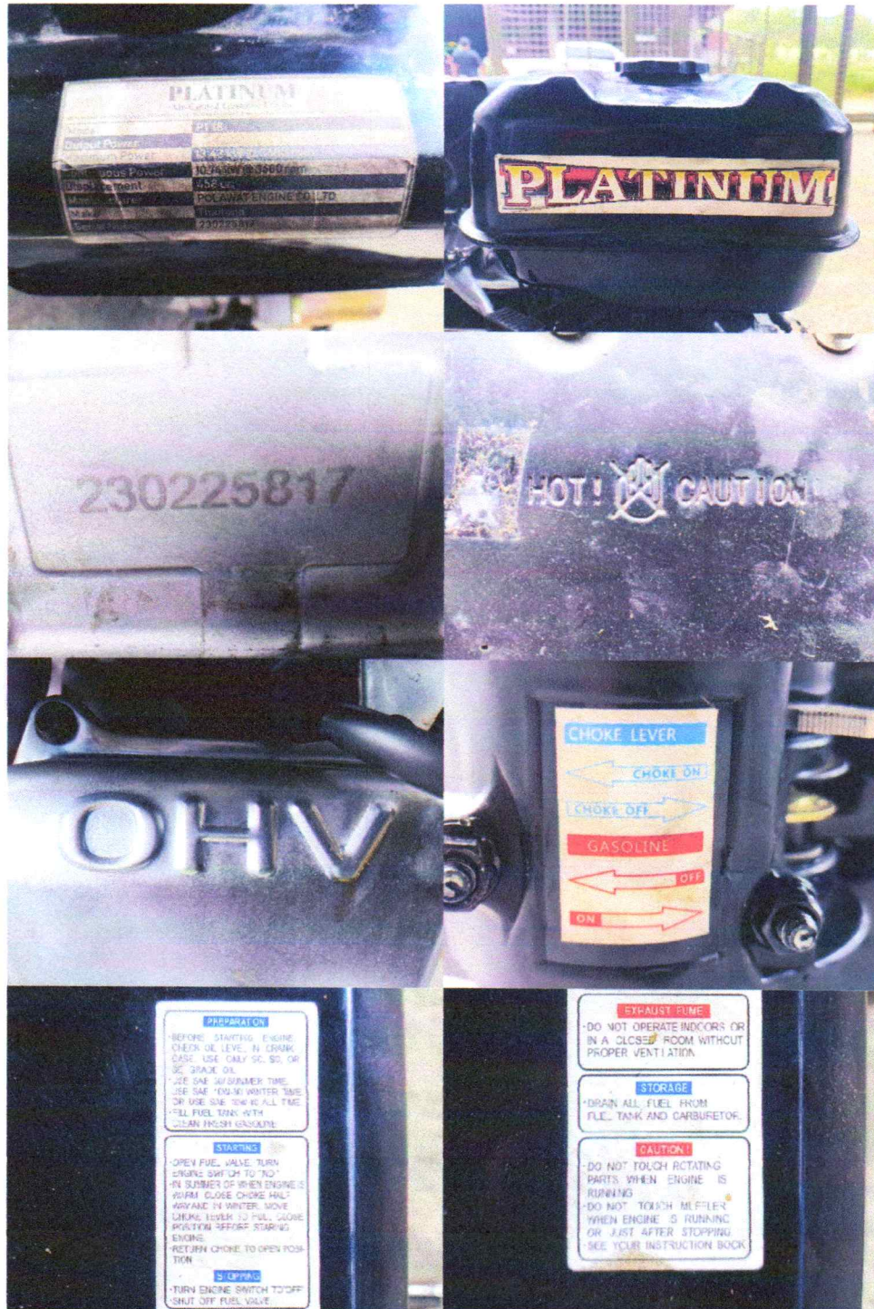
Figure 2. Components nameplate, markings, warning notices of Internal Combustion Engine PLATINUM PT18.
